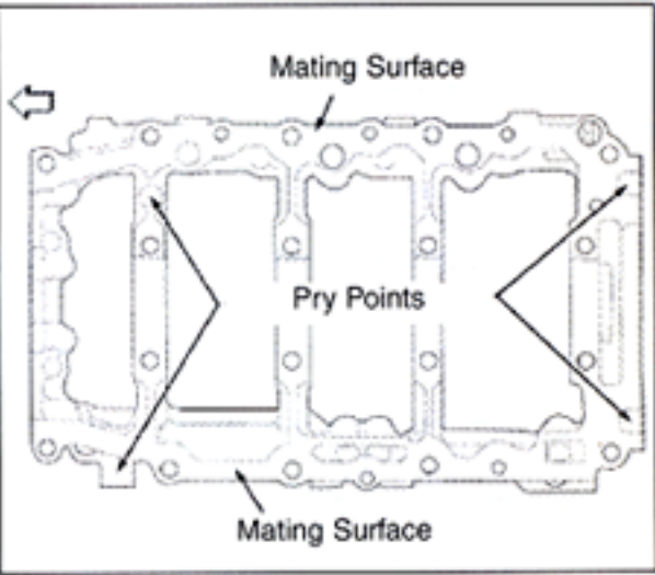
Figure 1 2003-'06 3.7L Chrysler/Jeep engine bedplate pry point locations.
