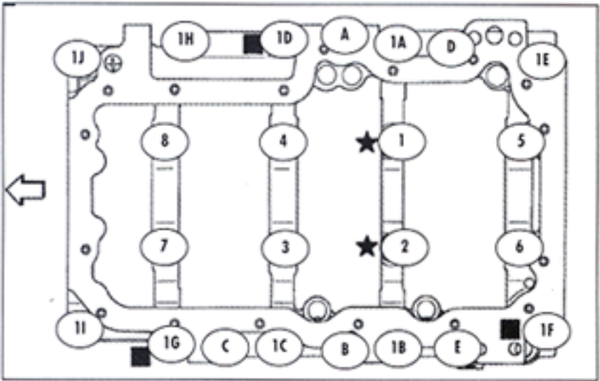
Figure 2 3.7L Chrysler/Jeep bedplate stud and dowel locations. Studs are indicated by stars; dowels by squares.
