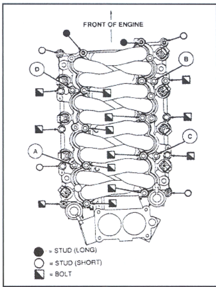
Figure 3 Tighten 1993-'96 Ford 4.6L intake manifold control bolts in sequence shown above.
