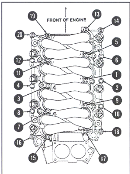
Figure 2 Tighten 1993-'96 Ford 4.6L intake manifold fasteners in sequence shown above.
