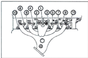
Figure 1 GM 4.2L torque sequence.
