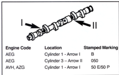
Figure 2 VW 2.0L engine cam identification.
