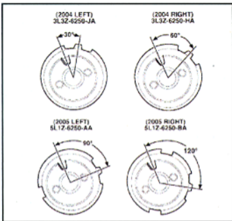
Figure 1 Camshaft identification is made by location of the VCT pin. At top, 2004 camshafts are shown; at bottom, 2005 camshafts are identified.
