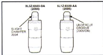
Figure 2 A groove in the lash adjuster will identify 2004 or 2005 components.
