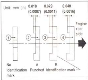
Figure 2 Three additional thickness plates are available for proper camshaft end play on Nissan 3.3L engines.
