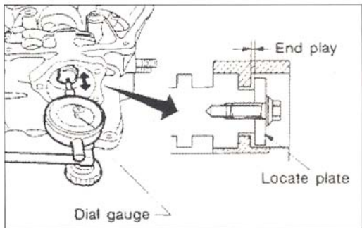
Figure 1 Measuring camshaft end play on Nissan 3.3L engines.
