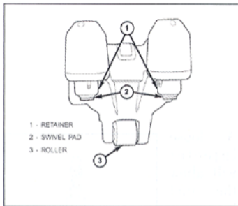
Figure 1 Rocker arm assembly for 1998-2002 Chrysler 3.2L and 3.5L engines. Noise complaints may be due to the associated movement between the exhaust swivel pad, retainer and rocker arm.
