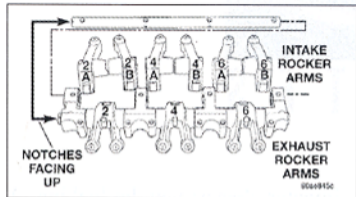
Figure 2 Rocker arm and stud location on 1998-2002 Chrysler 3.2L and 3.5L engines.
