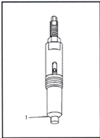
Figure 1 2001-2004 GM 6.6L diesel injectors may leak, allowing coolant into the combustion chamber if the injector sleeve seal is dirty or damaged.
